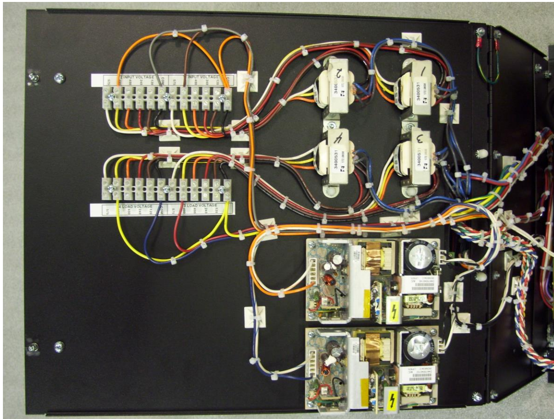
Rear (internal power supplies, potential transformers, voltage selection blocks shown)
