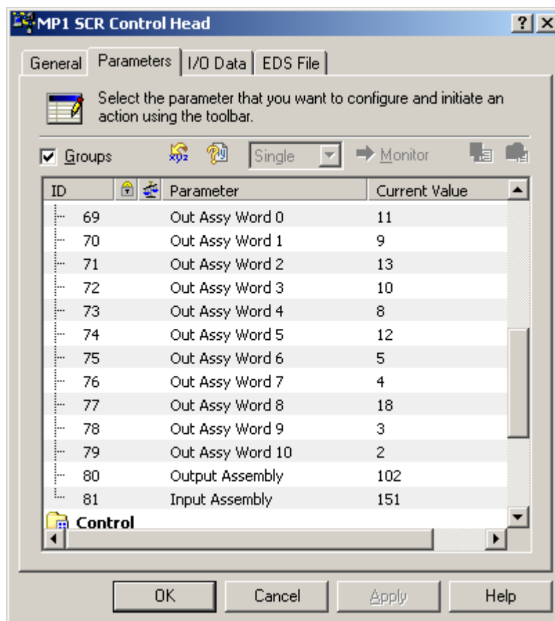
Figure 30 I/O Assembly Settings
