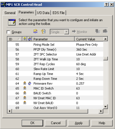
Figure 32 RSNetWorx Parameter Screen by Parameter Number
