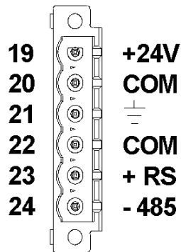
Figure 18 RS-485 Terminals
