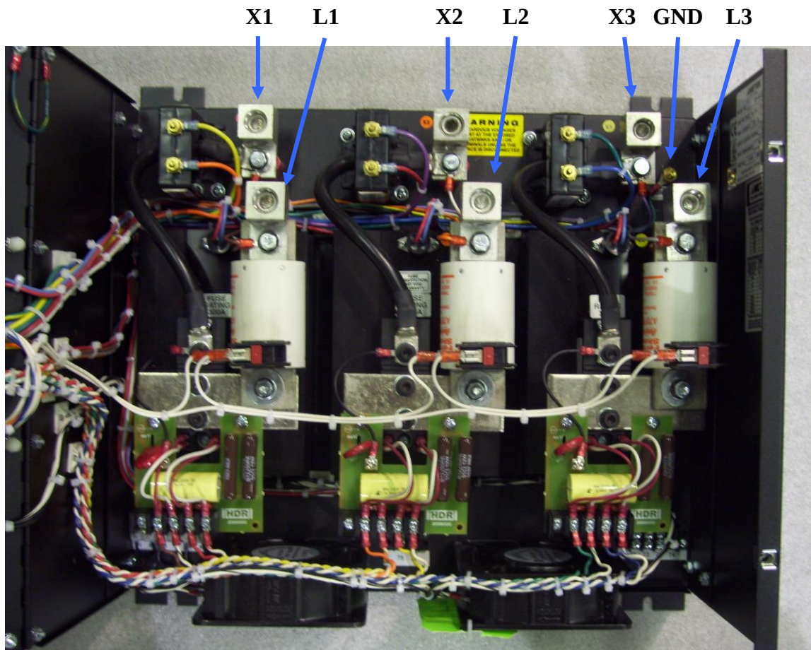
Figure 22 Wiring: L1, L2, L3, X1, X2, X3, GND. Refer to labels on other size units.
