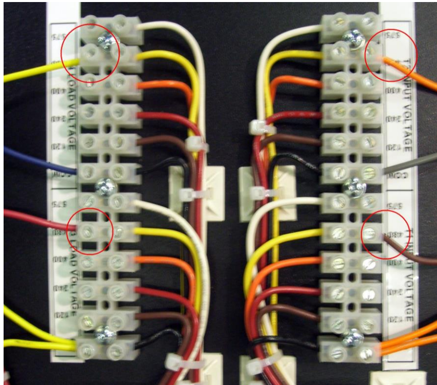
Figure 25 Wiring: Verity/Revise T1, T2, T3 & T42 Transformer Taps
