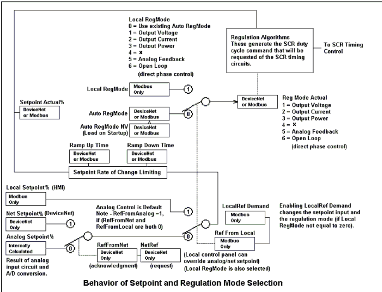
Figure 7 Diagram of the Setpoint and Regulation Logic
