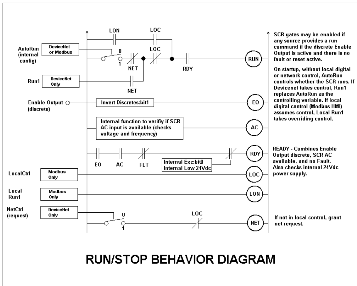
Figure 5 Run/Stop Control Logic.
