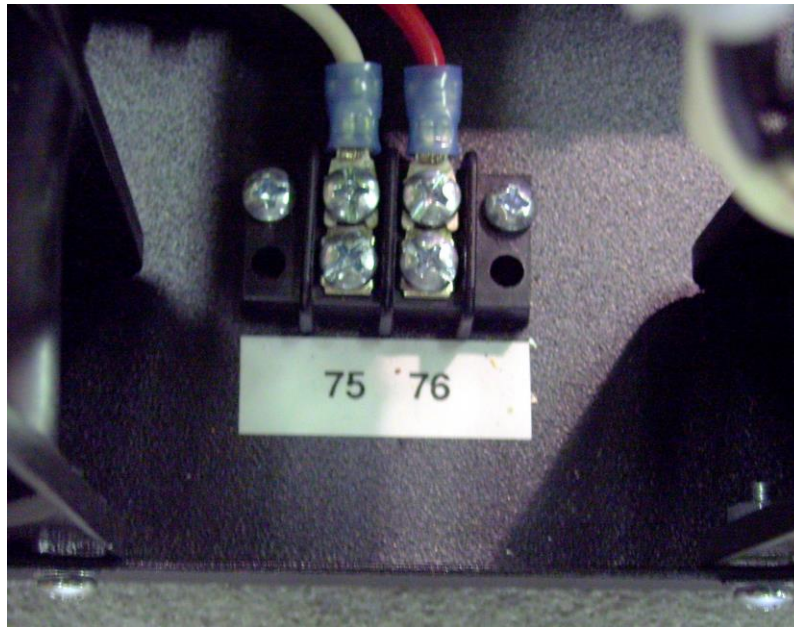
Figure 23 Wiring: Terminals 75-76 – Optional Current Transformer
