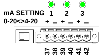
Figure 16 mA Transmitter Terminals.
