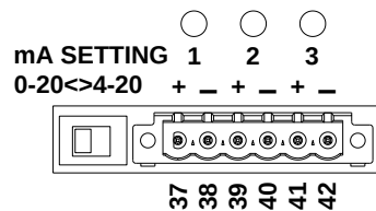
Figure 27 Wiring: Front – Three mA Drivers
