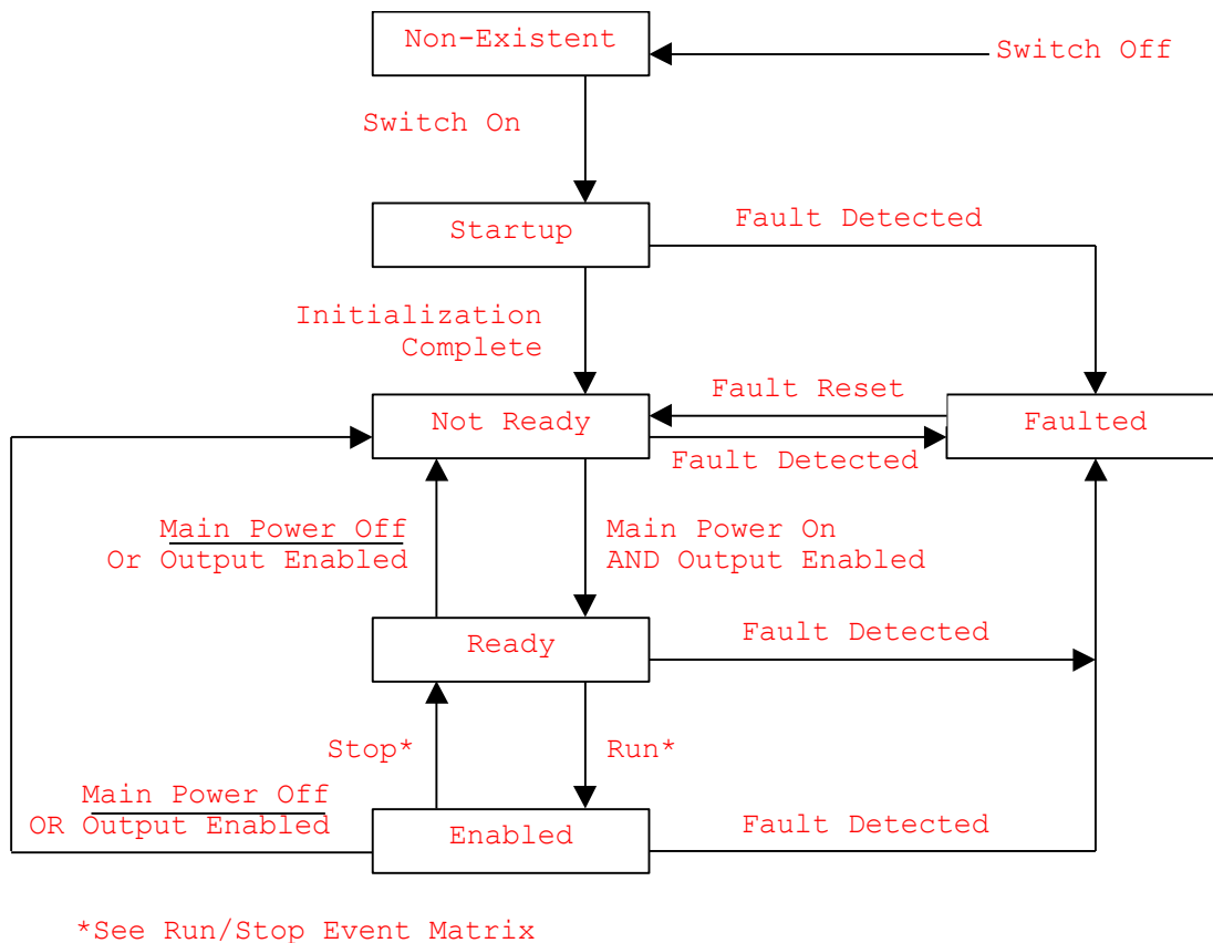
Figure 34 SCR Control Supervisor Behavior
