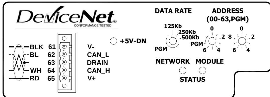
F Figure 19 DeviceNet Section, Front Panel.
