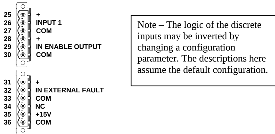
Figure 26 Wiring: Front – INPUT1, ENABLE OUTPUT, EXTERNAL FAULT
