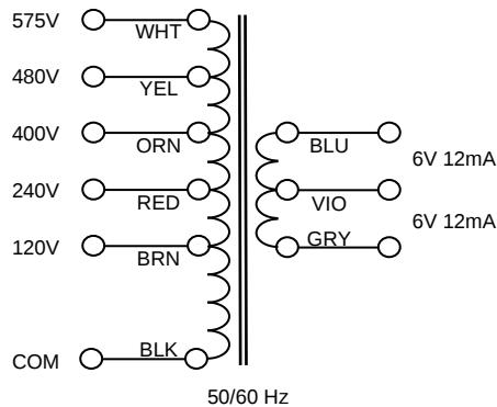
Figure 12 Voltage Potential Transformer
