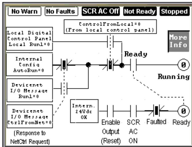
Figure 6 HMI Example Screen of Run/Stop Ladder Diagram.
