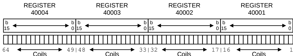
Figure 35 Map of Overlapping Modbus Coils and Registers
