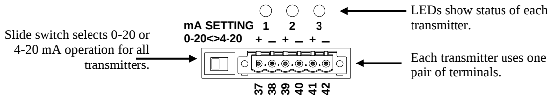
Figure 14 0-20/4-20 mA Transmitter Terminals
