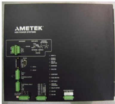
Figure 20 MP3 SCR DeviceNet Head (front, rear)
