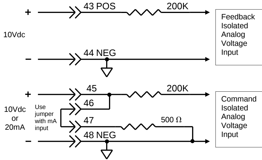
Figure 11 Analog Input Terminals
