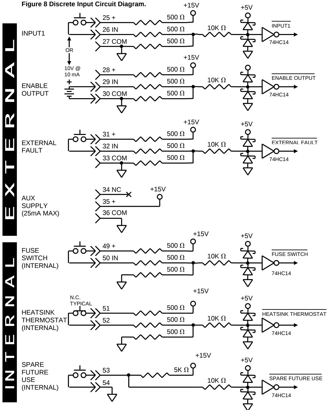
Figure 8 Discrete Input Circuit Diagram.
