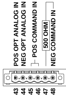
Figure 28 Wiring: Front – Analog In – COMMAND Setpoint
