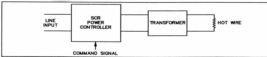
Figure 1 - Typical SCR controlled "Hot Wire" circuit
