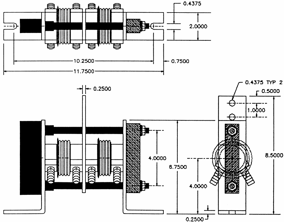
A typical dual SCR water-cooled chill block assembly. (Drawing courtesy of Value Engineered Products)
